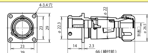
NAW-20 ■ -Ad(F)M □
