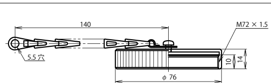
64EUMW-4RM
