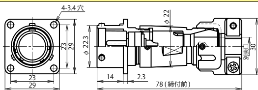
NAW-20 ■ -Ad(F)MK □
