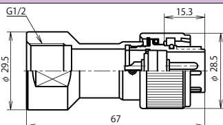
NAW-20 ■ -GPM1/2 (注)
