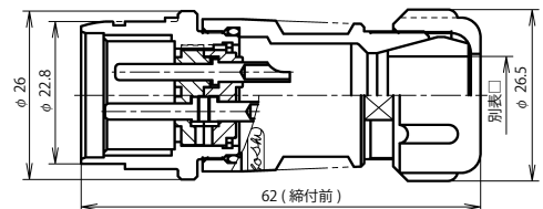
NEW-20 ■ -AdM □
