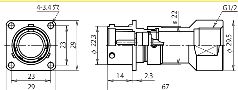
NAW-20 ■ -GAd(F)M1/2 (注)
