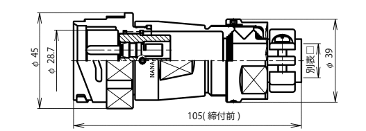
BWC-32 ■ -AdM □
