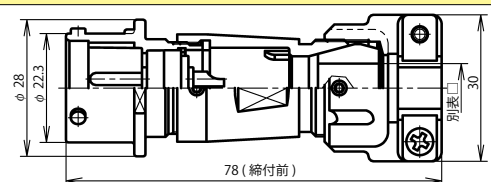
NAW-20 ■ -AdMK □
