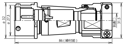
NAW-24 ■ -AdMK □
