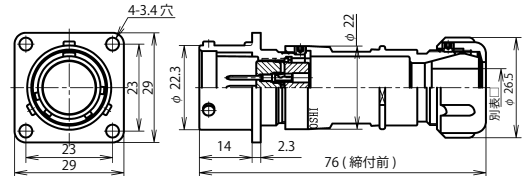
NAW-20 ■ -Ad(F)M □
