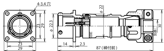
NAW-20 ■ -Ad(F)MK □
