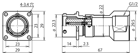
NAW-20 ■ -GAd(F)F1/2 (注)
