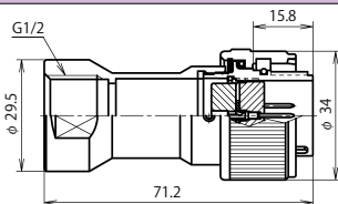
NAW-24 ■ -GPM1/2 (注)
