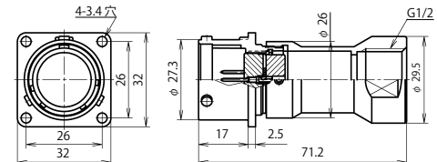
NAW-24 ■ -GAd(F)M1/2 (注)
