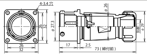
NAW-24 ■ -Ad(F)M □
