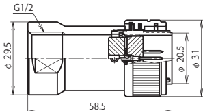
NR-24 ■ -GPM1/2 (注)
