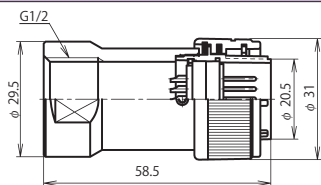
NR-24 ■ -GPM1/2 (注)
