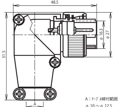
NR-20 ■ -LPM
