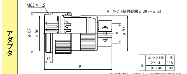
NCS-60 ■ -Ad
