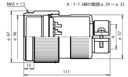
NCS-60 ■ -AdF
