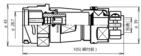
BWC-32 ■ -AdM □
