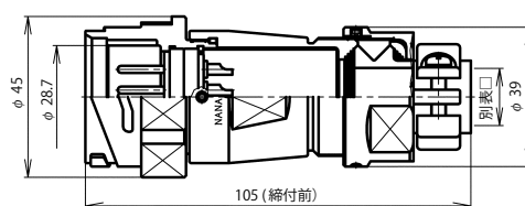
BWC-32 -AdM
